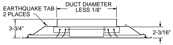
Side View Detail, SF Frame
