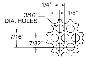
Perforated Pattern Detail (51% free area)
