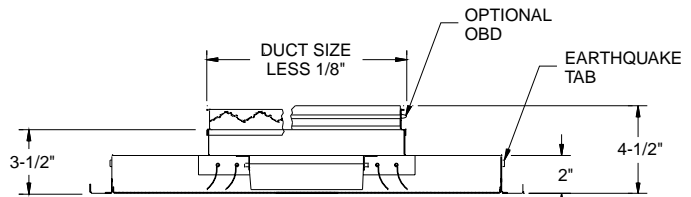
Side View/Damper Detail, SF Frame
