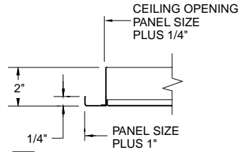
Frame SF (Surface Mount) *minimum ceiling opening 23-1/4"
