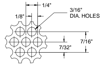
Perforated Pattern Detail (51% free area)
