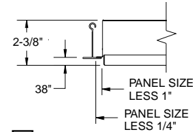
Frame TG (Tegular)
