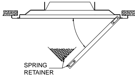
Face Hinge Detail
