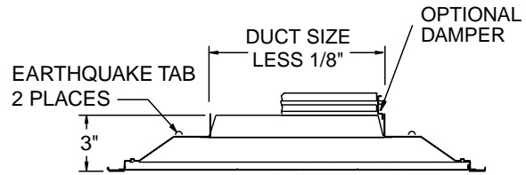
Side View/Damper Detail, SF Frame
