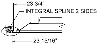
Frame PL (Spline)
