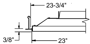
Frame TG** (Tegular)
