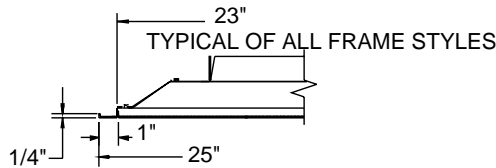
Frame SF (Surface Mount) *minimum ceiling opening 23-1/4"
