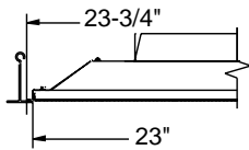
Frame LT (Lay-in-T-Bar)
