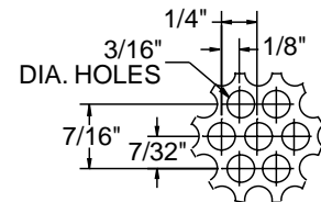
Perforated Pattern Detail (51% free area)
