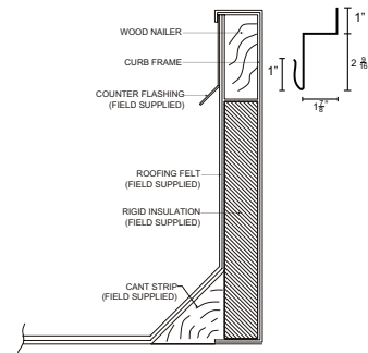
TYPICAL FLASHING DETAIL
