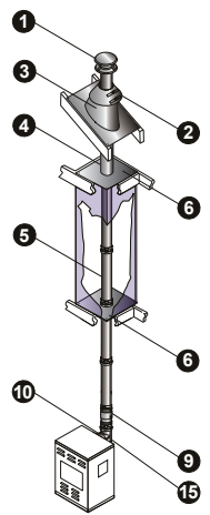
Multi-Story Installation
