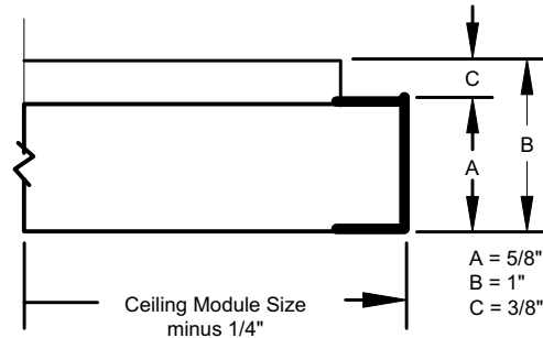
U - Frame Detail
