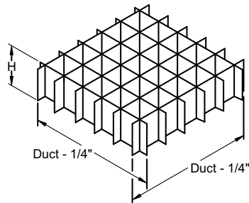
C - Core Only Detail
