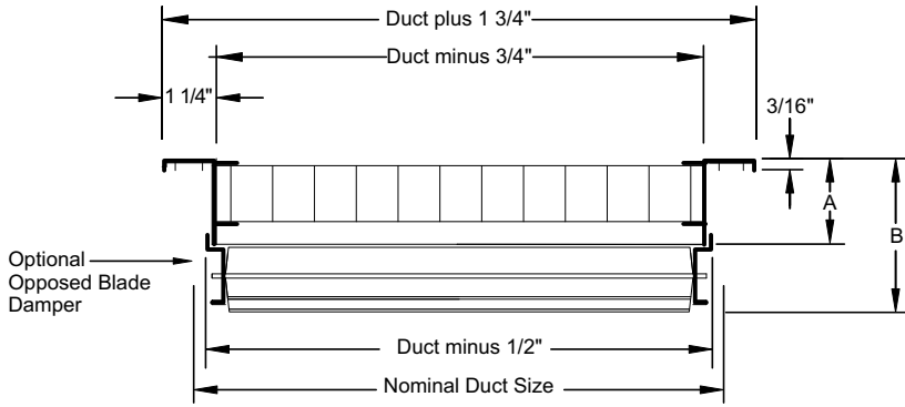
Side View / Damper Detail, SF Frame
