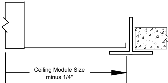
LT - Lay in T - Bar Detail
