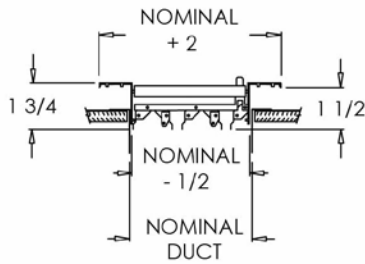
951 O (Extruded Frame)
