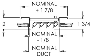
951 (Stamped Steel One Piece Frame)
