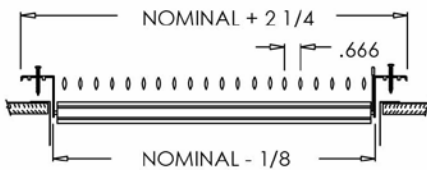
951 O (Extruded Frame)
