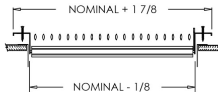
951 (Stamped Steel One Piece Frame)
