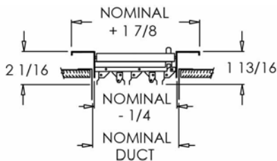
951-O (Stamped Steel One Piece Frame)
